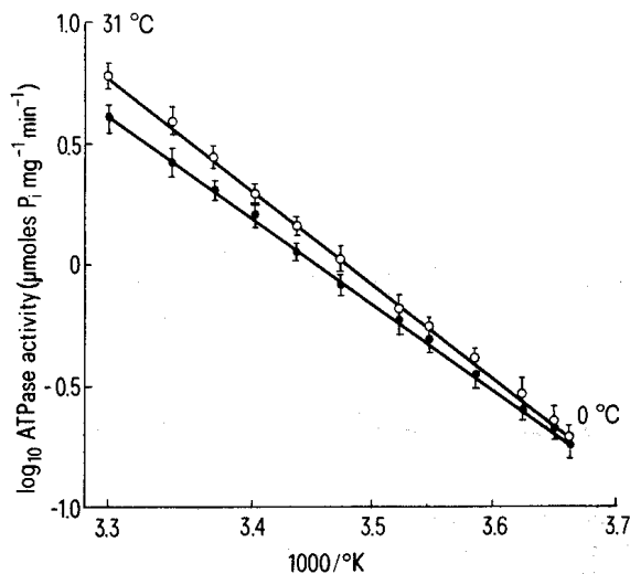
Fig. 1. Arrhenius plots of \text{Mg}^{2+}\text{Ca}^{2+} -myofibrillar ATPase activities from warm- and cold-acclimated brook trout ( Salvelinus fontinalis ). +4 °C acclimated fish; +24 °C acclimated fish. Means \pm 1 SEM of 8 fish. Assay conditions given in text. Slopes of regression lines are not statistically significant ( p > 0.05 ).
