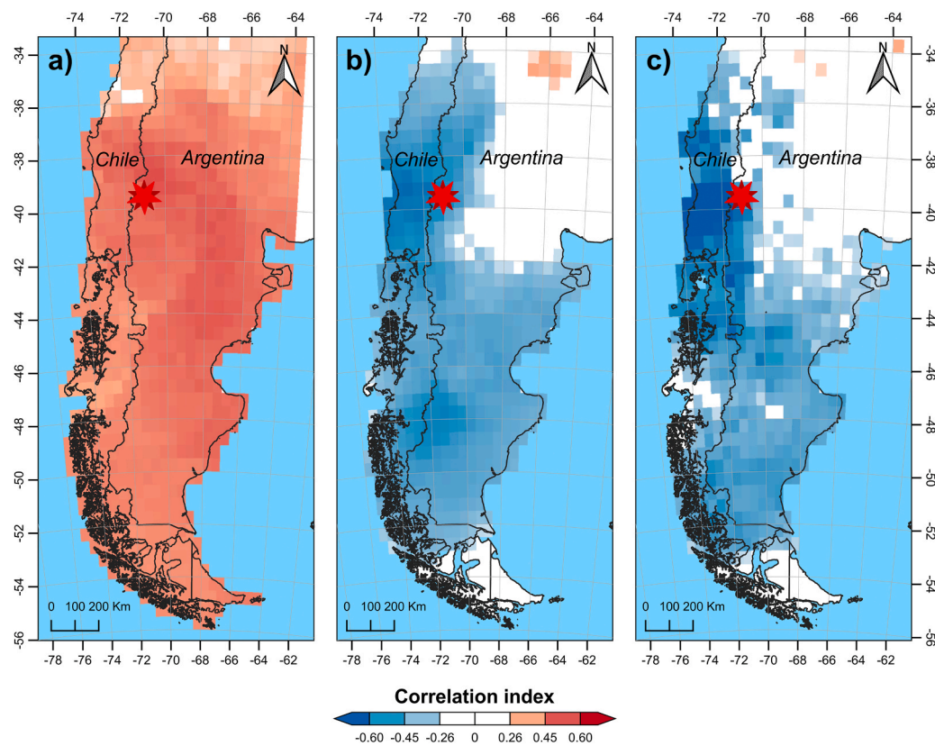
Fig. 8. Extensive spatial correlation patterns between BI chronologies and gridded climate data for a) summer CRU TS4.07 temperature (DJF), b) CRU TS4.07 spring precipitation (SON) and c) summer CRU scPDSi over the 1950–2005 common period. In (a) the most extensive correlation spatial pattern was obtained with the mean of the residual DBI chronologies, in (b) with the mean of the residual EWBI chronologies, and in (c) with the mean of residual LWBI chronologies. The maps were created with the KNMI Climate Explorer facilities and displayed with QGIS Desktop (v 3.4.13). Coloured gridded areas over the SA continent reflect significance at p < 0.05 . The red double star icon points the sampling site.
