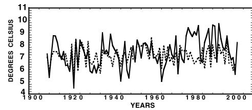
Figure 2. Actual (solid line) and estimated (dashed line) Nome May–August temperatures from 1909–2001 based on SP-MXD chronology, including both calibration (1909–1950) and verification (1951–1970) periods. Note that estimates after ca. 1970 tend to underpredict actual values (calibration ar^2 declines from 42% for 1909–1950 to 38% for 1909–70 and 23.2% for 1909–2001). The ar^2 for the verification period is 26%, with a positive RE of 0.20 in verification. Additional tests: calibration 1909–1920: ar^2 67%, verification 1921–1950: RE = 0.31; calibration 1921–1950: ar^2 38%; verification 1909–1920: RE = 0.40.
