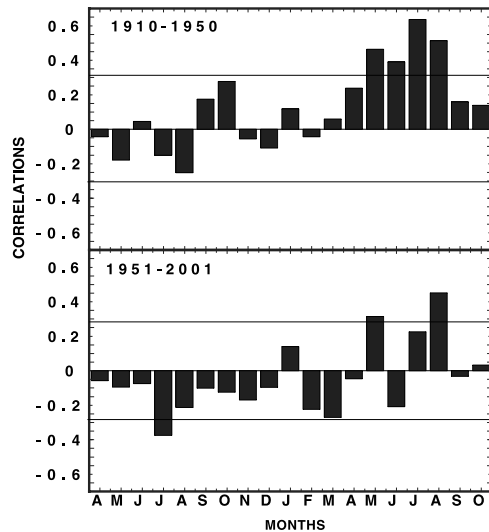
Figure 1. Correlation of SP-MXD chronology with Nome, SP mean monthly temperatures for prior and current growth year. Top: 1910–1950; bottom: 1951–2001. Horizontal lines denote 95% confidence levels. Nome temperature data from Global Historical Climate Network (vol. 2) [Peterson and Vose, 1997] and A. Lloyd (personal communication, 2003).
