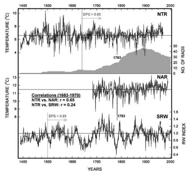
Figure 3. Top line: May–August NTR extending from 1389–1970 (recent decades truncated, see text), based on 1909–1950 model. Thick lines shows smoothed values. Horizontal lines indicate mean values. Chronology based on 3 SP sites: Death Valley (65.19°N, 162.27°W, 239m), Alpine View (65.11°N, 162.18°W, 282m) and Hey Bear (65.22°N, 162.22°W, 229m) [D'Arrigo et al. , submitted to Holocene , 2004]. Gray shading shows changing sample size over time, which ranges from 1–7 radii prior to 1640. Inferences of past climate prior to ca. 1640 should be interpreted with caution. Low value in 1783 is labeled. Middle line: May–August NAR [Jacoby et al. , 1999]. Bottom line: SRW series [D'Arrigo et al. , submitted to Holocene , 2004]. Vertical lines in SP records indicate acceptable EPS cutoff of 0.85 [Cook and Kairiukstis, 1990].
