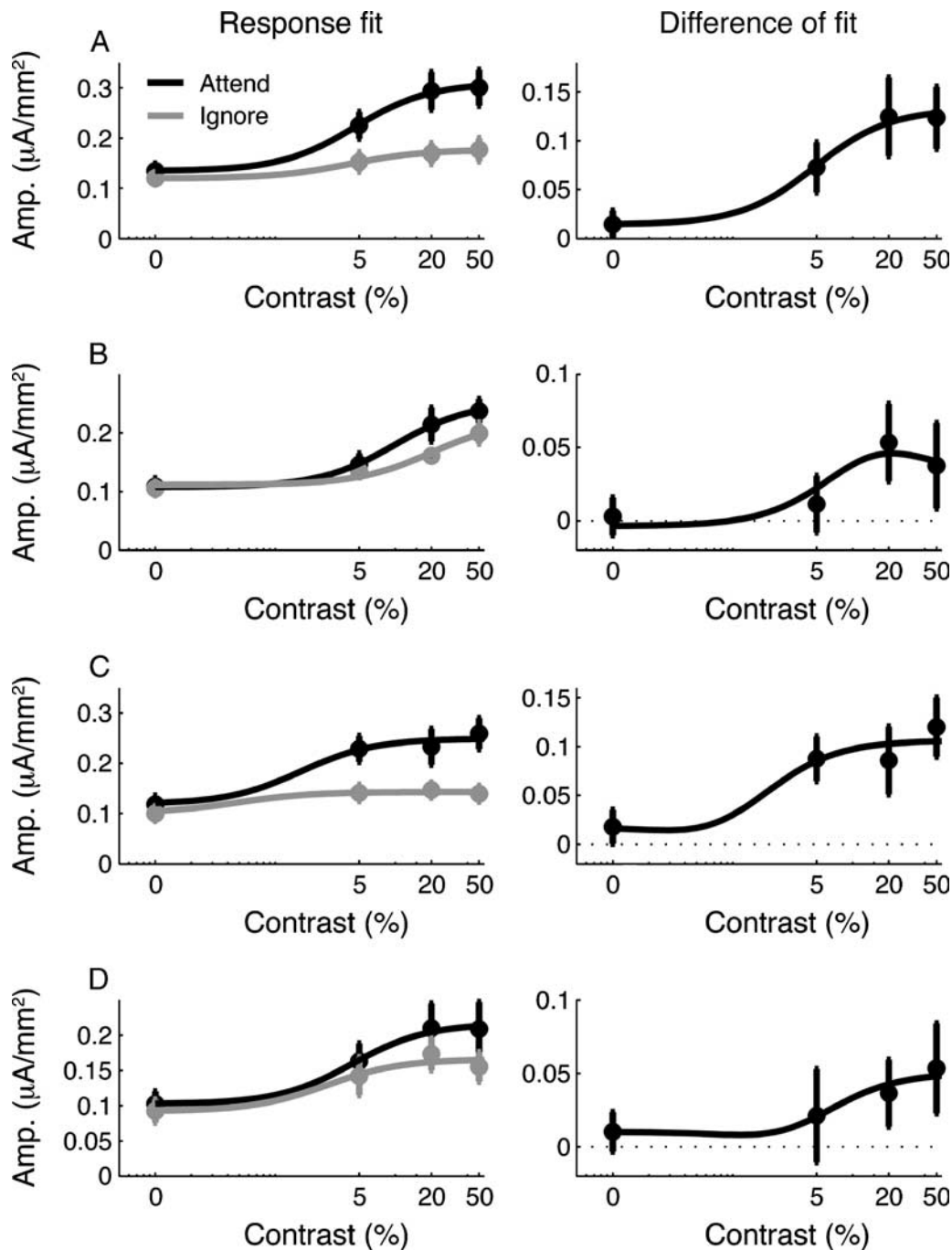
Figure 4. Fits of the hyperbolic ratio model of the contrast response function to the response amplitudes for attend and ignore. The left column is the fit of the attend (black) and ignore (gray) amplitudes of the current density, and the right column is their difference. (A) V1, (B) hV4, (C) hMT+, (D) IPS. V1, hMT+, and IPS display response gain, while hV4 displays evidence of contrast gain. Error bars are \pm 1 SEM.
