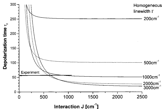
FIG. 12. The theoretical dependence of depolarization time \tau , on interchromophore interaction for C_3 -three-chromophore molecular system. The depolarization time obtained from experimental is also shown by an arrow.
