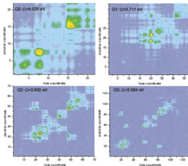
FIG. 5. (Color) Second lowest energy modes of the four dendrimer generations showing excitations located on the dendrons. The color coding is as in Fig. 4.
