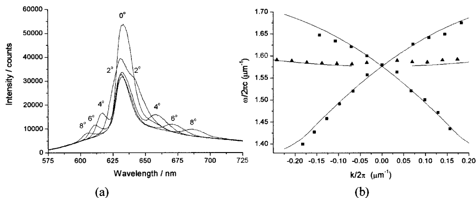
FIG. 4. (a) Angle dependent PL spectrum of a directly patterned OC 1 C 10 -PPV film and (b) PL peak positions as a function of in-plane wavevector and frequency (points) and theoretical fit (lines).
