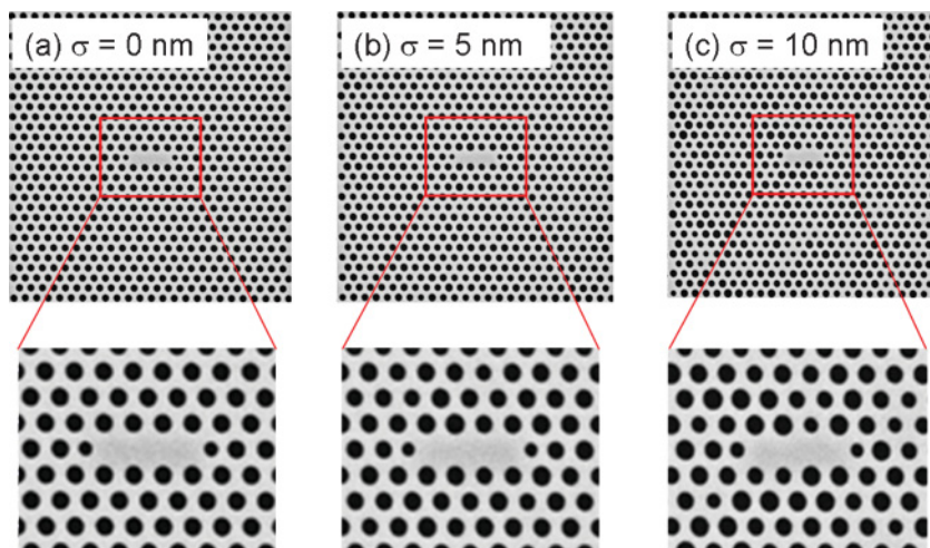
FIG. 1. (Color online) SEM images of cavities with nominal disorder parameter \sigma = 0, 5, and 10 nm, respectively.
