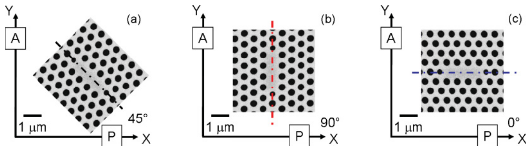
FIG. 6. (Color online) The figure shows three different orientations of the cavity axis with respect to the polarizer P : (a) 45^\circ , (b) 90^\circ , and (c) 0^\circ .
