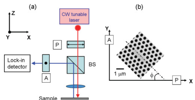
FIG. 2. (Color online) (a) Scheme of the experimental setup for cross-polarized CW light scattering measurements. (b) SEM image of an L3 PhC nanocavity, showing its orientation with respect to polarizer and analyzer.
