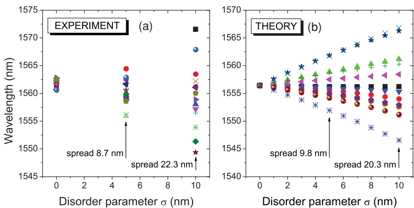
FIG. 10. (Color online) (a) Experimental behavior and (b) theoretical calculation of cavity mode wavelength versus the disorder parameter \sigma for 15 different disorder distributions. The nearby hole shift is fixed to \Delta x/a = 0.16 .
