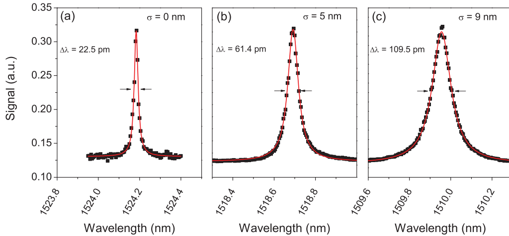
FIG. 3. (Color online) Cross-polarized scattering spectra (square dots) for three cavities with a = 420 nm, r/a = 0.3 , \Delta x/a = 0.16 , \Delta r/r = -0.06 but with different amount of disorder (0, 5, and 9 nm, respectively). Best fits with Fano lineshapes are also shown (continuous lines).
