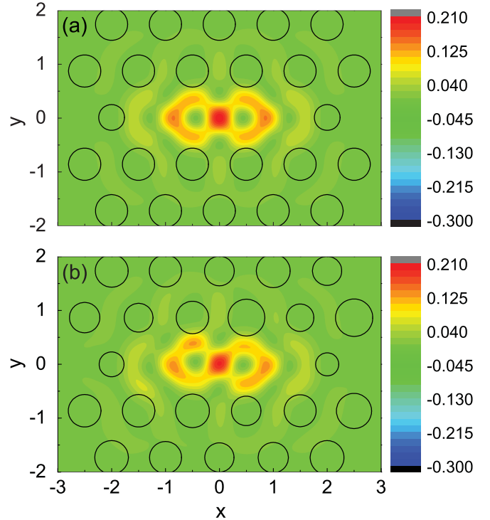
FIG. 5. (Color online) Squared electric field profiles for the cases of (a) nominal zero disorder and (b) nominal \sigma = 10 nm disorder. The random variations of the radii can be noticed in (b).
