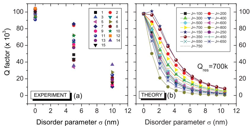
FIG. 9. (Color online) (a) Experimental behavior and (b) theoretical calculation of Q factors versus the disorder parameter \sigma for 15 different disorder distributions. The nearby hole shift is fixed to \Delta x/a = 0.16 .
