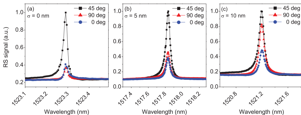
FIG. 7. (Color online) Scattering spectra for three cavities with \Delta x/a = 0.16 and disorder parameter (a) \sigma = 0 nm, (b) \sigma = 5 nm, and (c) \sigma = 10 nm, respectively. Spectra are measured for three different sample orientations: 45^\circ (square dots), 90^\circ (triangular dots), and 0^\circ (circular dots).
