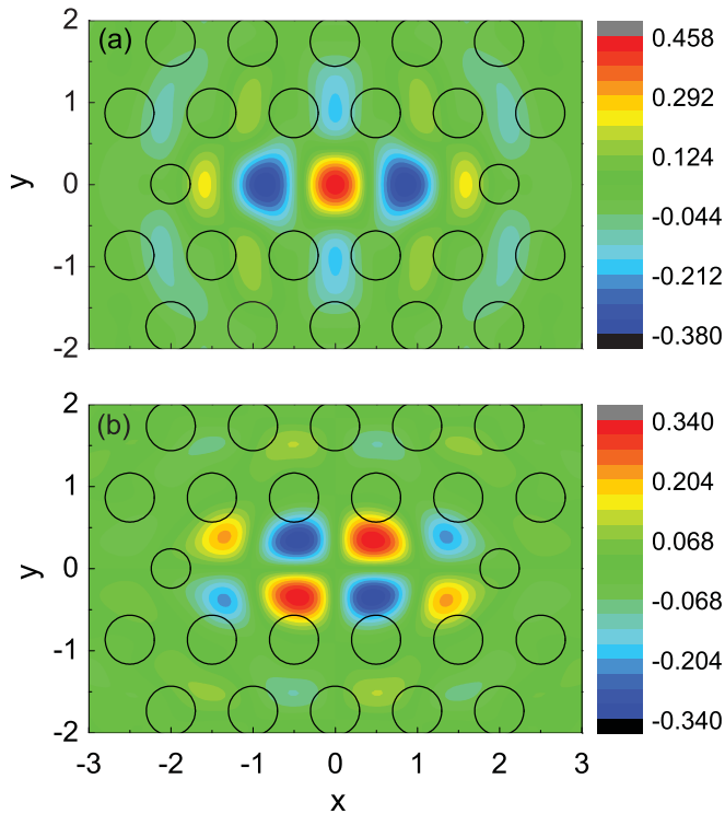
FIG. 4. (Color online) Imaginary part of the electric field (a) E_y and (b) E_x .
