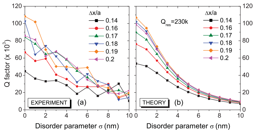
FIG. 8. (Color online) (a) Experimental behavior of the Q factors versus the disorder parameter \sigma for six series of cavities with different nearby hole shifts \Delta x/a . (b) Theoretical calculation of Q versus \sigma , assuming an intrinsic Q_{\text{res}} = 230 \times 10^3 (see text). It should be noted that each experimental datapoint corresponds to a different disorder distribution, whereas the distribution is the same for each of the theoretical curves and is scaled with \sigma .
