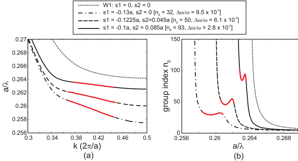
Fig. 3. (a) Calculated dispersion curves and (b) group indices, for the fundamental mode of the modified W1 PhC waveguides with s1 and s2 values indicated by the blue circles in Fig. 2(b). The thick solid red line represents the flat band slow light region. The group index – bandwidth product was around 0.3 in all cases. The result of W1 waveguide is also presented for comparison
