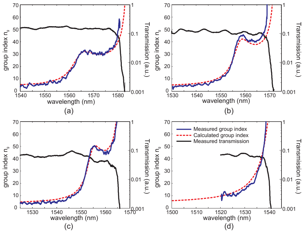
Fig. 5. Measured transmission spectra (black solid lines) and experiment (blue solid lines) and calculated (red dashed lines) group index of the PhC waveguides with s1 and s2 values indicated in Fig. 2(b): (a) s1 = -52 nm and s2 = 0 nm, (b) s1 = -50 nm and s2 = 12 nm, and (c) s1 = -48 nm and s2 = 16 nm. The flat band group index and the corresponding group index – bandwidth products are n_g = 32.5 for n_g(\Delta\omega/\omega) = 0.29 , n_g = 44 for n_g(\Delta\omega/\omega) = 0.31 , and n_g = 49 for n_g(\Delta\omega/\omega) = 0.3 respectively. The result of a normal W1 PhC waveguide is also presented for comparison (d).
