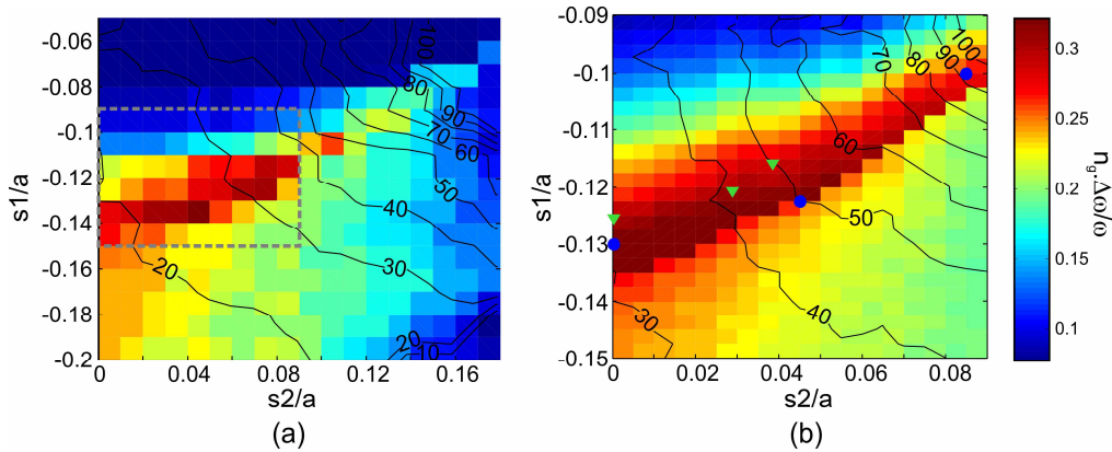
Fig. 2. Systematic maps of (a) 2D and (b) 3D calculations of the group index – bandwidth product as a function of s_1 and s_2 . The color plot and the contours represent n_g(\Delta\omega/\omega) and n_g respectively. The rectangle in Fig. 2(a) indicates the calculation region of Fig. 2(b). The three blue circles and green triangles in Fig. 2(b) indicate the calculation points in Fig. 3 and the experimental points in Fig. 5 respectively.
