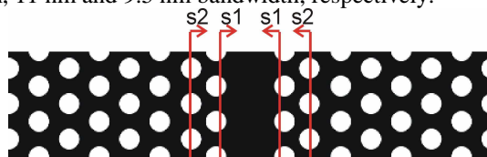
Fig. 1. Geometry of the modified W1 PhC waveguides: the first and second rows of holes are displaced symmetrically about the waveguide axis. The displacements relative to the unmodified lattice (red lines) are given by s_1 and s_2 , where shifts toward the waveguide centre are defined to be positive. Here, s_1 < 0 and s_2 > 0 , as used throughout this paper.
