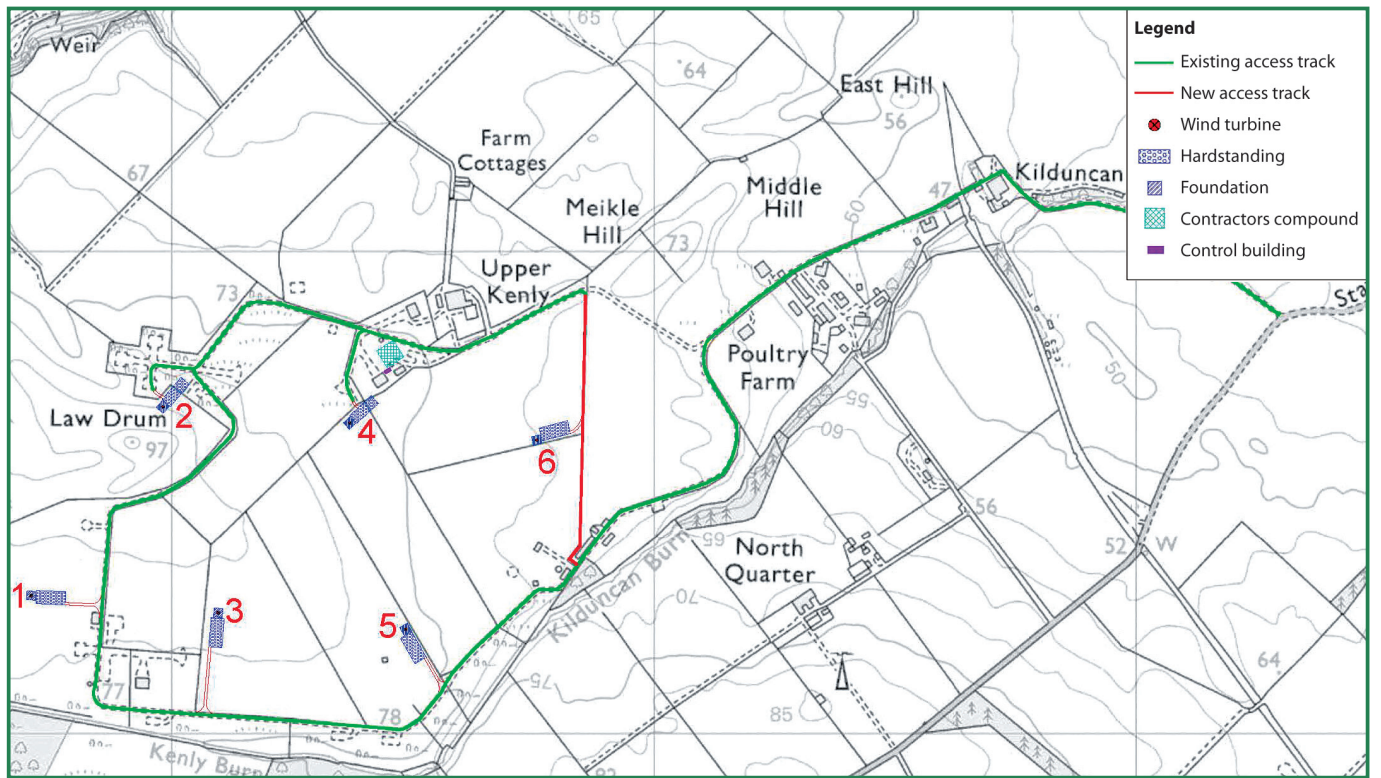
Proposed Kenly wind farm layout plan
